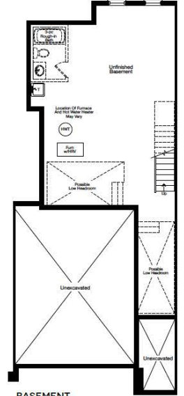
BASEMENT ELEVATION A & B
