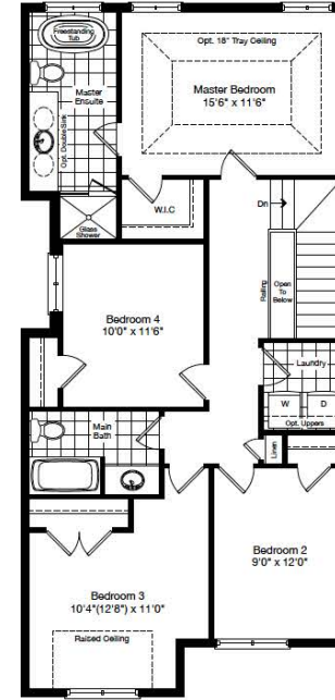
OPTIONAL SECOND FLOOR W/4 BEDROOMS ELEVATION A
