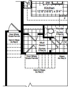
PARTIAL GROUND FLOOR ELEVATION A & B WHEN PAIRED WITH TH-01, ON BLOCK 133 LOT 5, BLOCK 139 LOT 3, BLOCK 140 LOT 3 ONLY
