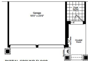
PARTIAL GROUND FLOOR ELEVATION B
