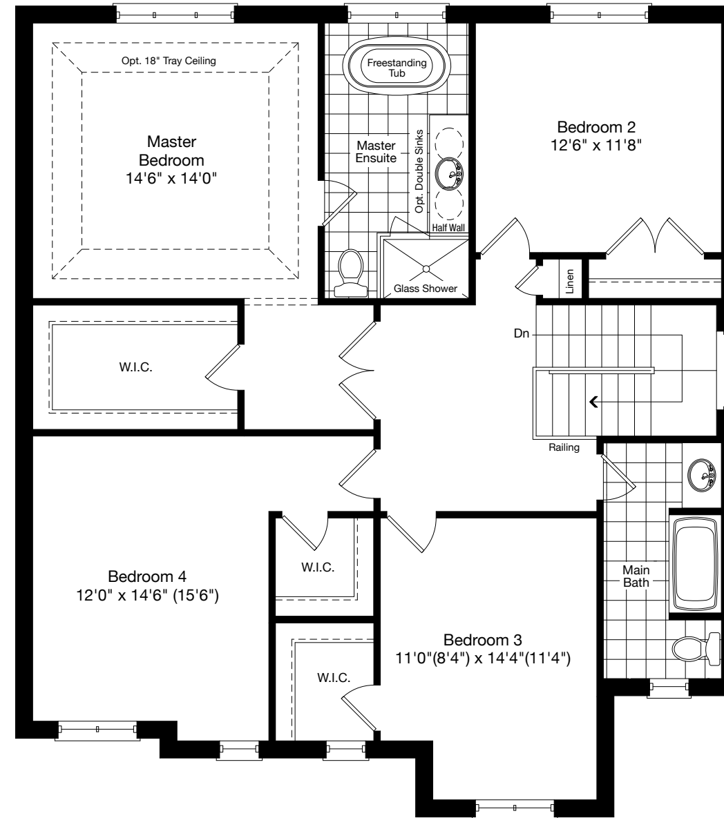
SECOND FLOOR ELEVATION A
