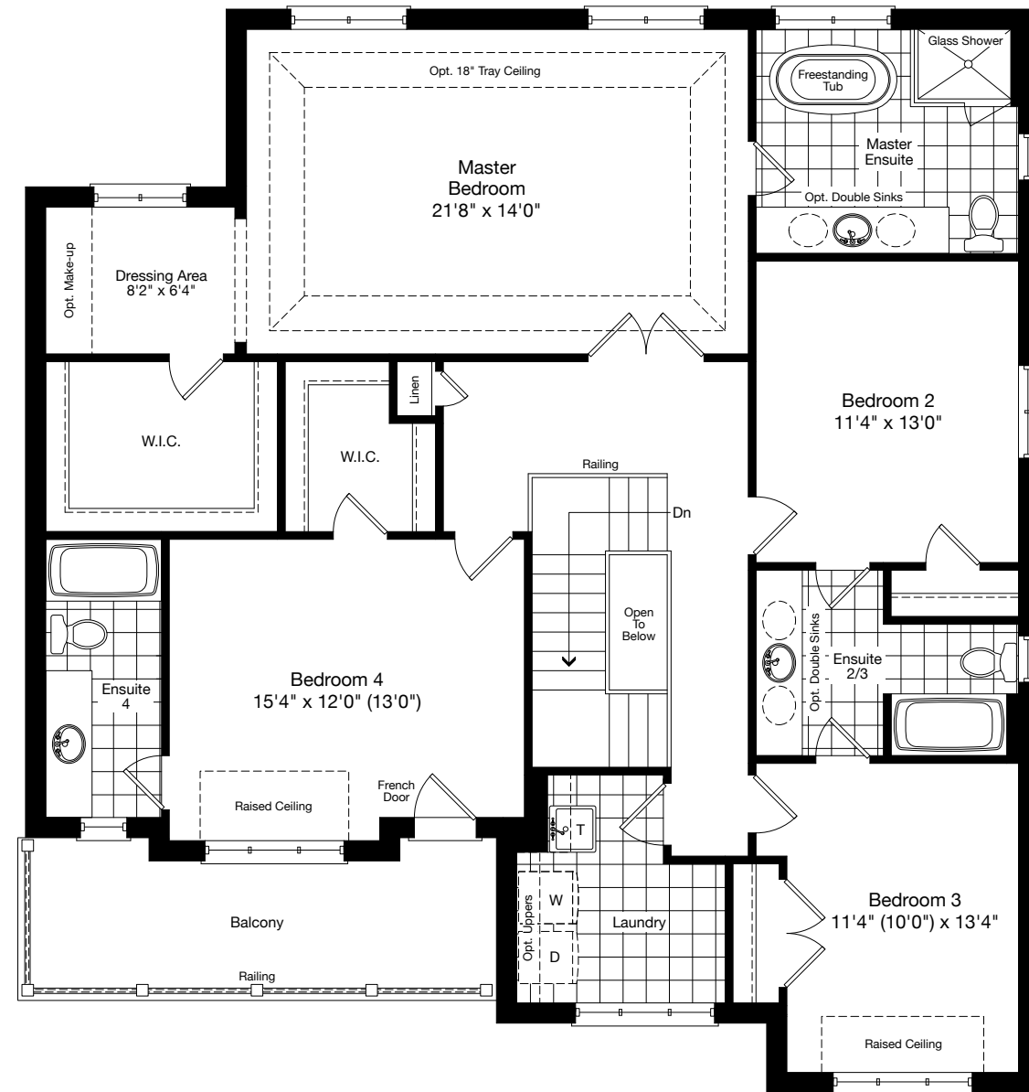
SECOND FLOOR ELEVATION A
