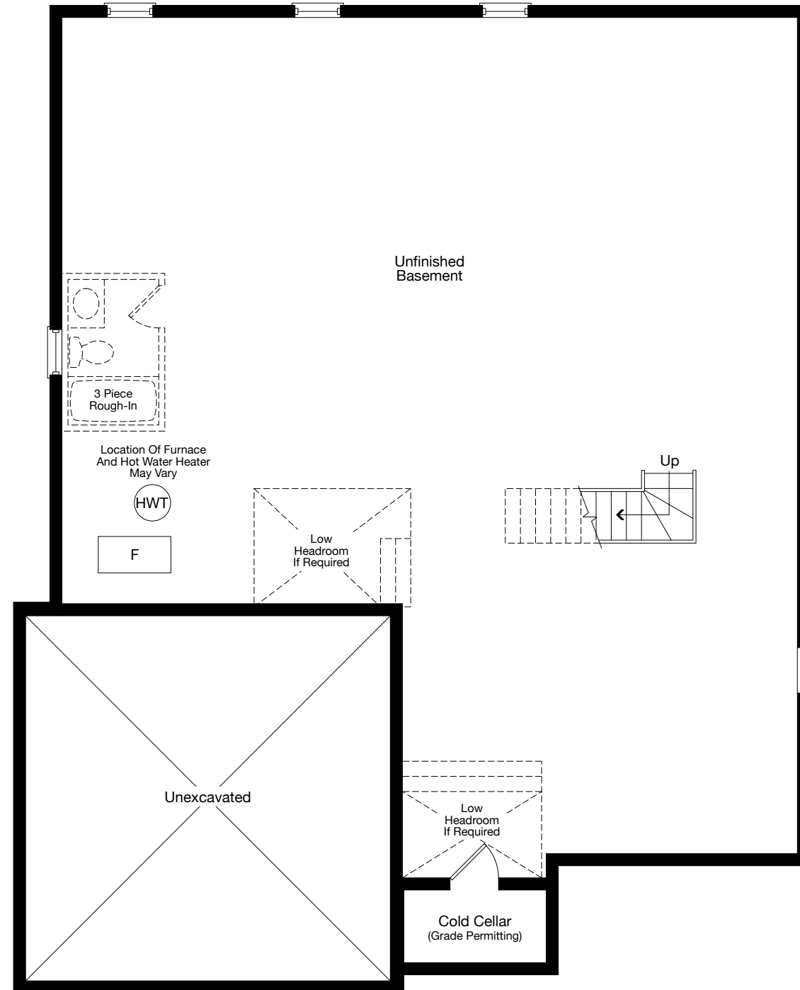
BASEMENT ELEVATION A & B
